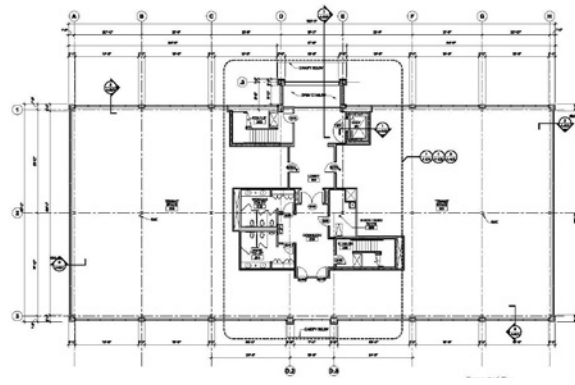
SECOND FLOOR OFFICE BUILDING 20,100 SF
